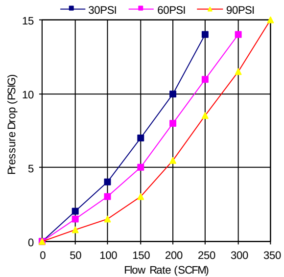
AF5000 Series Filter Flow Rate VS Pressure Drop @ 30, 60, 90 PSI Supply Pressure
