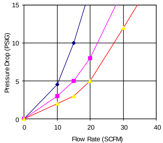
AF2000 Series Filter Flow Rate VS Pressure Drop @ 30, 60, 90 PSI Supply Pressure
