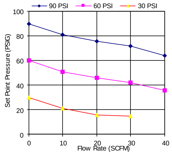
AC2000 Series Filter Regulator Lubricator Flow Rate VS Set Point Pressure Supply Pressure 100 PSI
