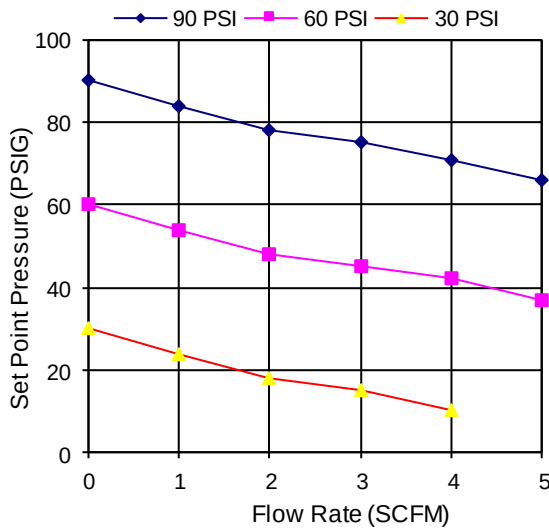
AC1000 Series Filter Regulator Lubricator Flow Rate VS Set Point Pressure Supply Pressure 100 PSI
