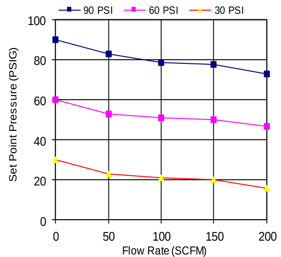
AC4000 Series Filter Regulator Lubricator Flow Rate VS Set Point Pressure Supply Pressure 100 PSI
