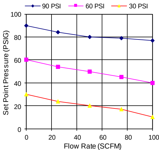
AC3000 Series Filter Regulator Lubricator Flow Rate VS Set Point Pressure Supply Pressure 100 PSI
