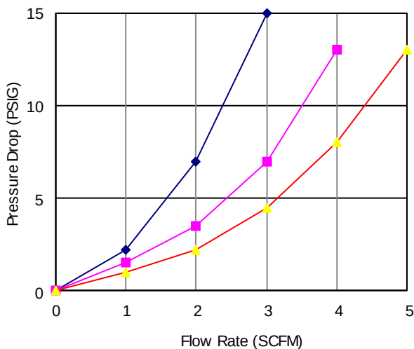
AF1000 Series Filter Flow Rate VS Pressure Drop @ 30, 60, 90 PSI Supply Pressure
