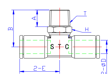
Branch Tee (BT)
