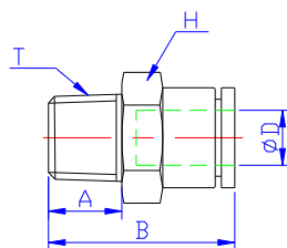
Male Connector (MC)
