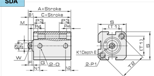
SDA 12-16, Female Thread
