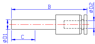
Tube Reducer (TR)
