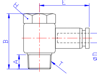
Universal Elbow (UE)
